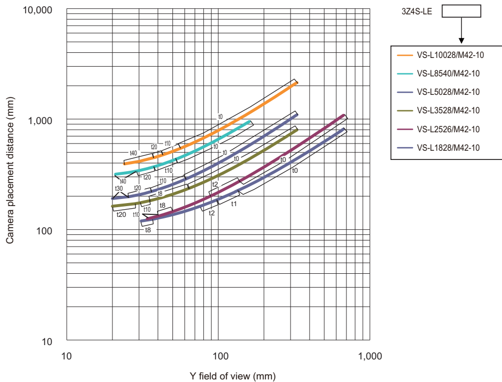
(h) High-speed Digital CMOS Camera (Standalone): FH-S□12 (Using 3Z4S-LE VS-L/M42-10 Series)
